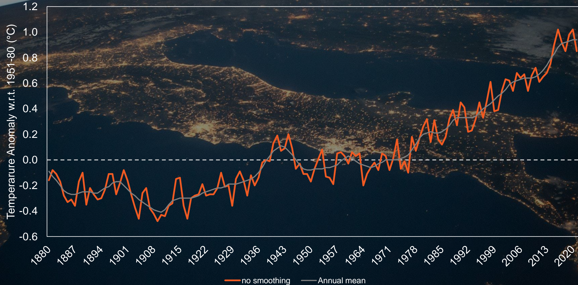
Global Annual Mean Surface Air Temperature Change
